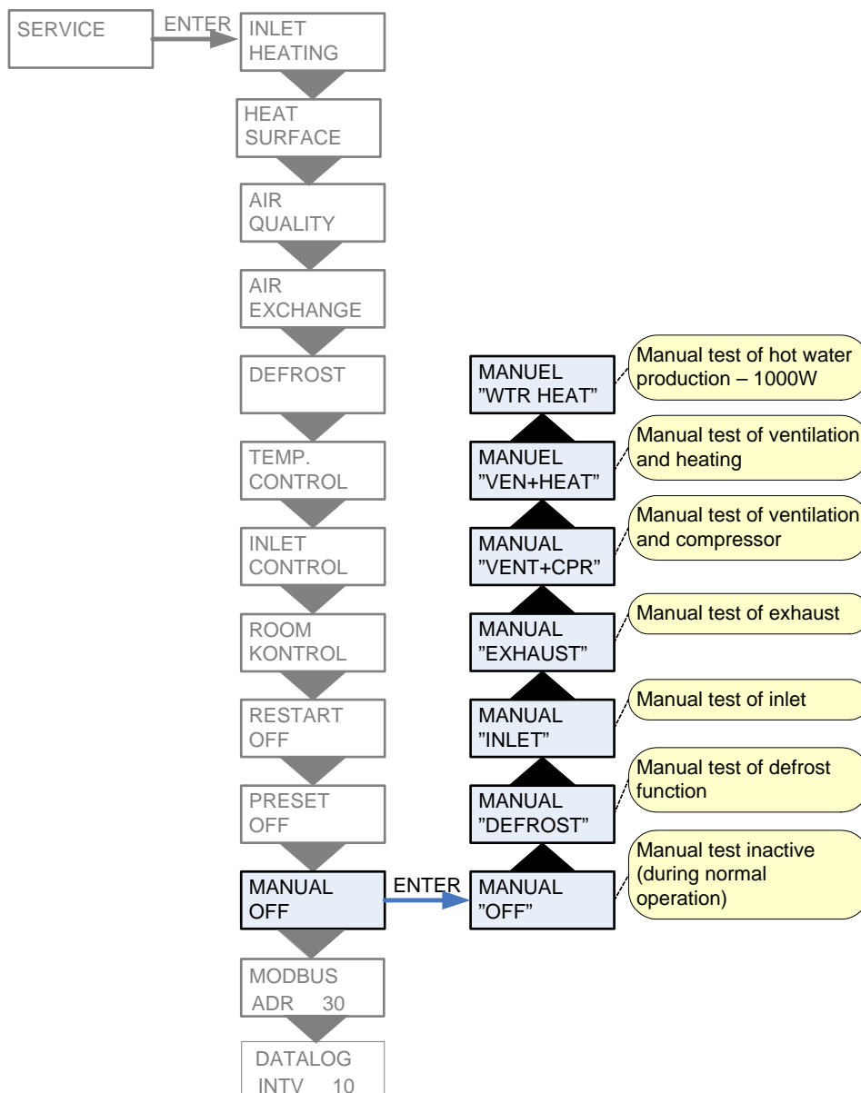
Figure 17: The "Manual" Menu
