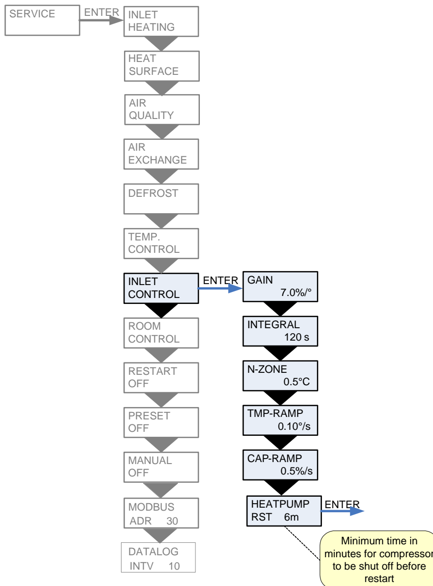
Figure 13: The "Inlet control" Menu
