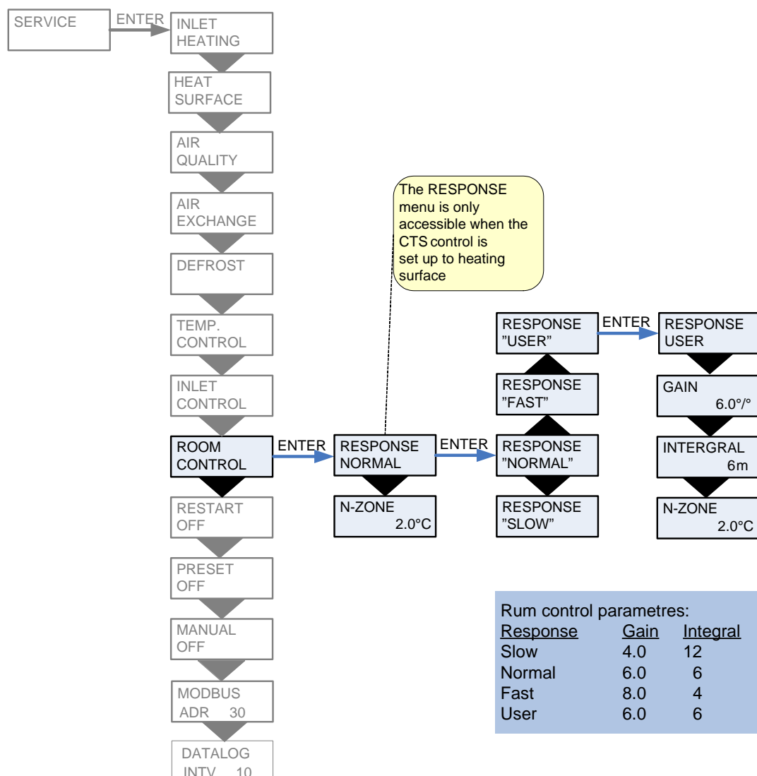
Figure 14: The "Room control" Menu
