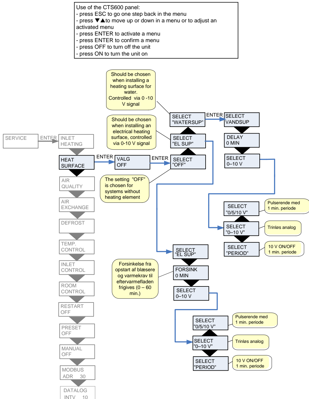
Figure 8: The “Central heating” menu
