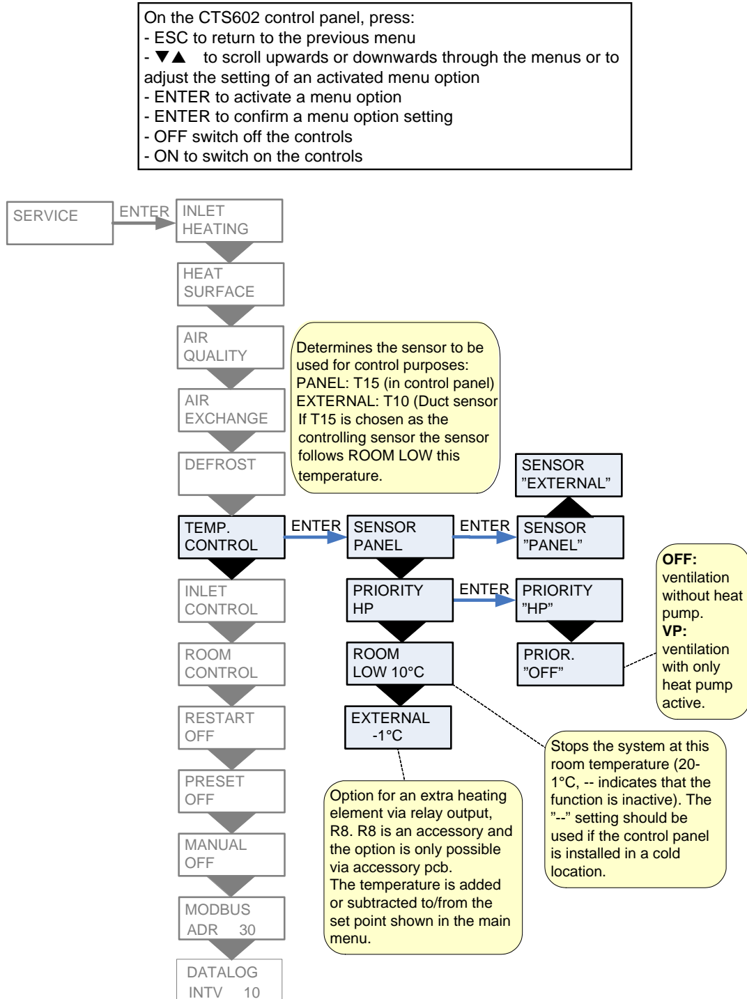
Figure 12: The "Temp. control" Menu
