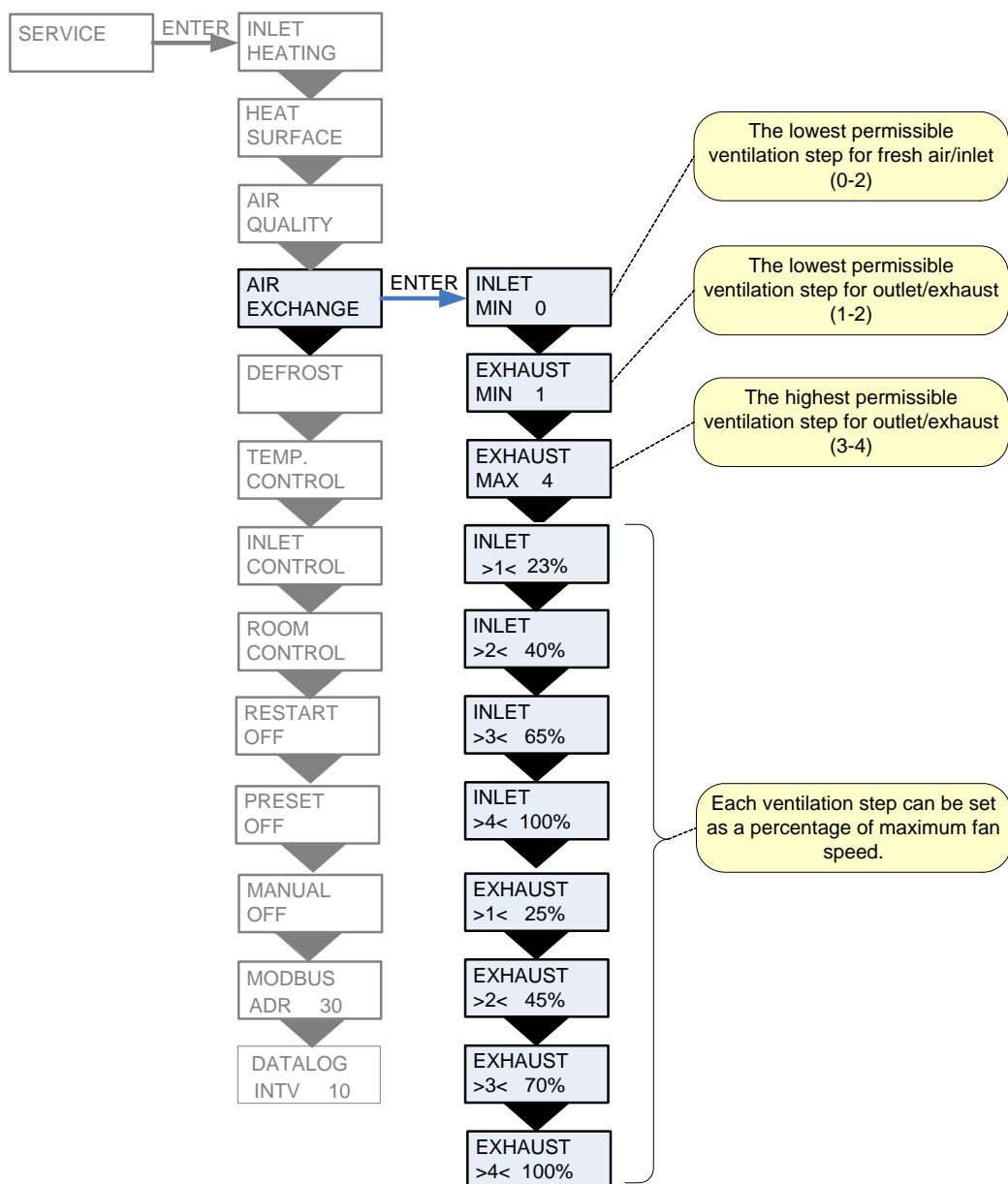
Figure 10: The "Air exchange" Menu
