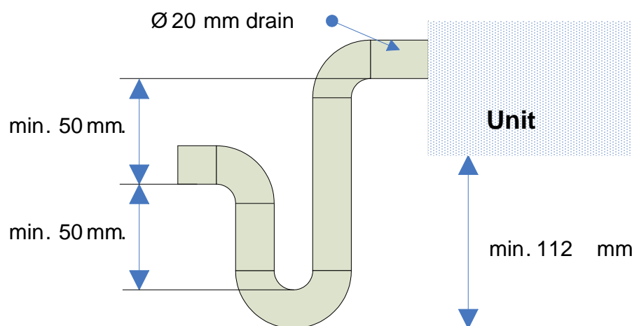
Figure 3: Condensation drain / water seal
