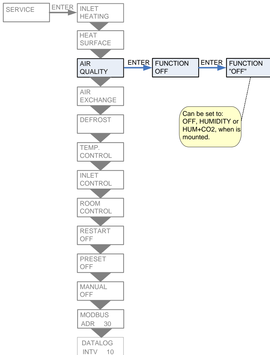
Figure 9: The "Air quality" Menu
