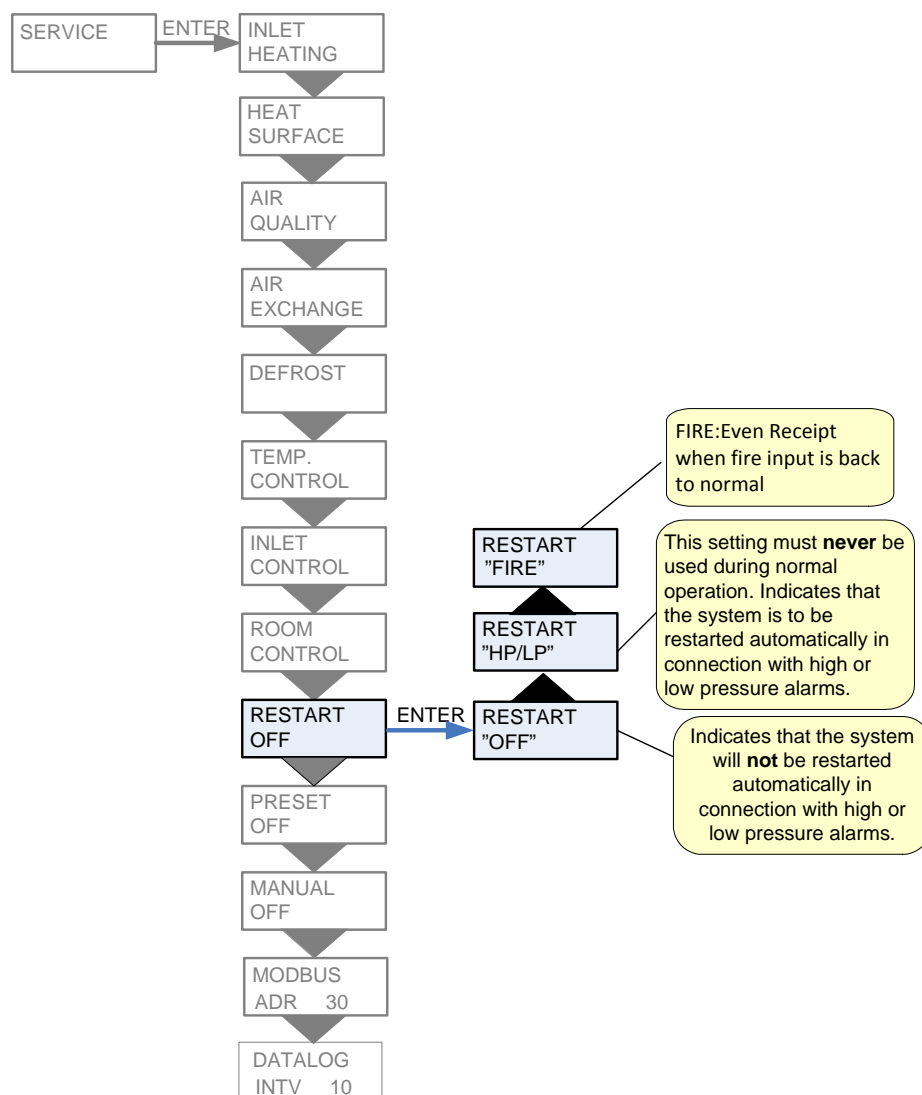
Figure 15: The "Restart" Menu
