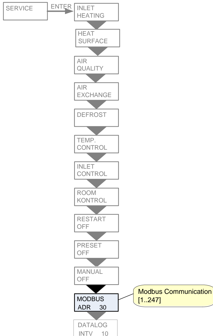
Figure 18: The "Modbus" Menu
