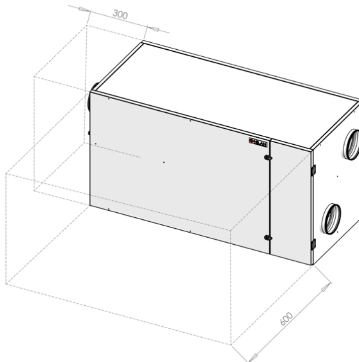
Figure 2: Mounting the Combi 302 Polar
