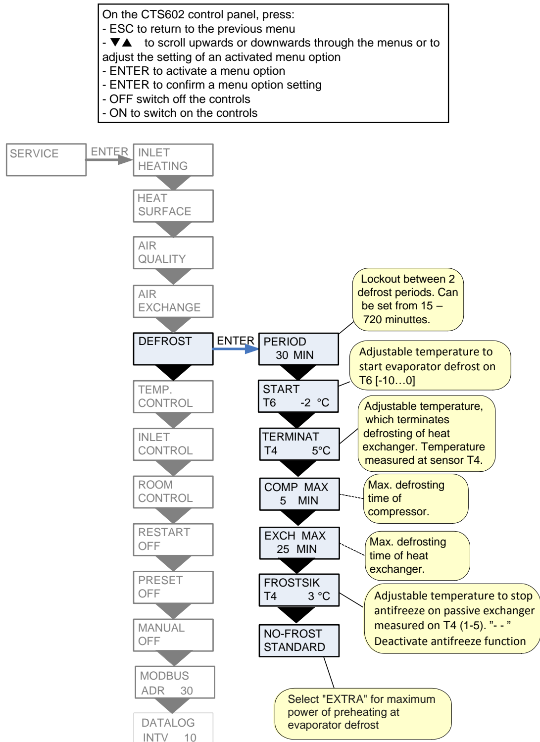
Figure 11: The "Defrost" Menu
