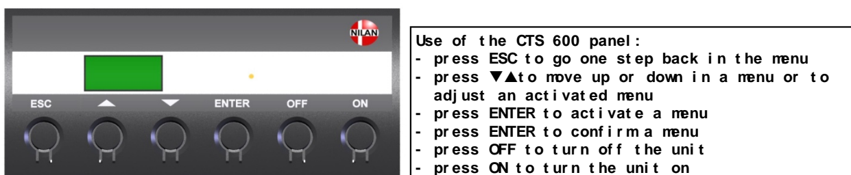
Figure 1: CTS 602 control
