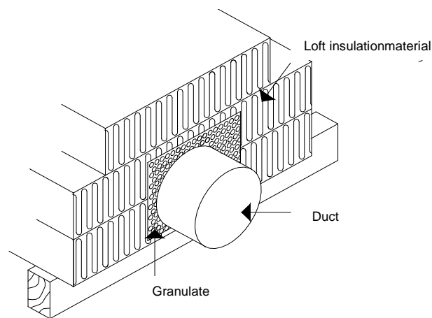
Figure 4: Insulation of ducting
