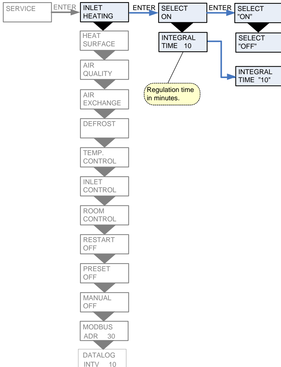
Figure 7: The "Inlet heating" Menu
